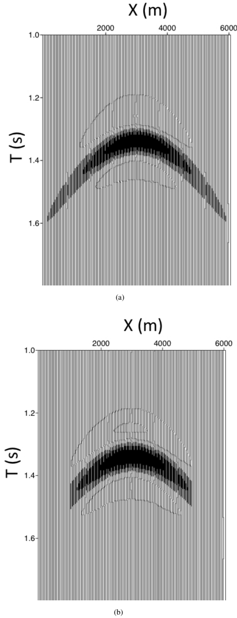
Figure 2: Vertical displacement for the model in Table 1 generated using (a) the reflectivity method and (b) the Kirchhoff scattering integral. The wavefield is excited and recorded on top of the model. The source is a vertical force at X = 3.0 km and the receivers are placed between X = 0.5 km and X = 5.5 km with a 50 m increment. The source signal is a Ricker wavelet with a central frequency of 10 Hz.
