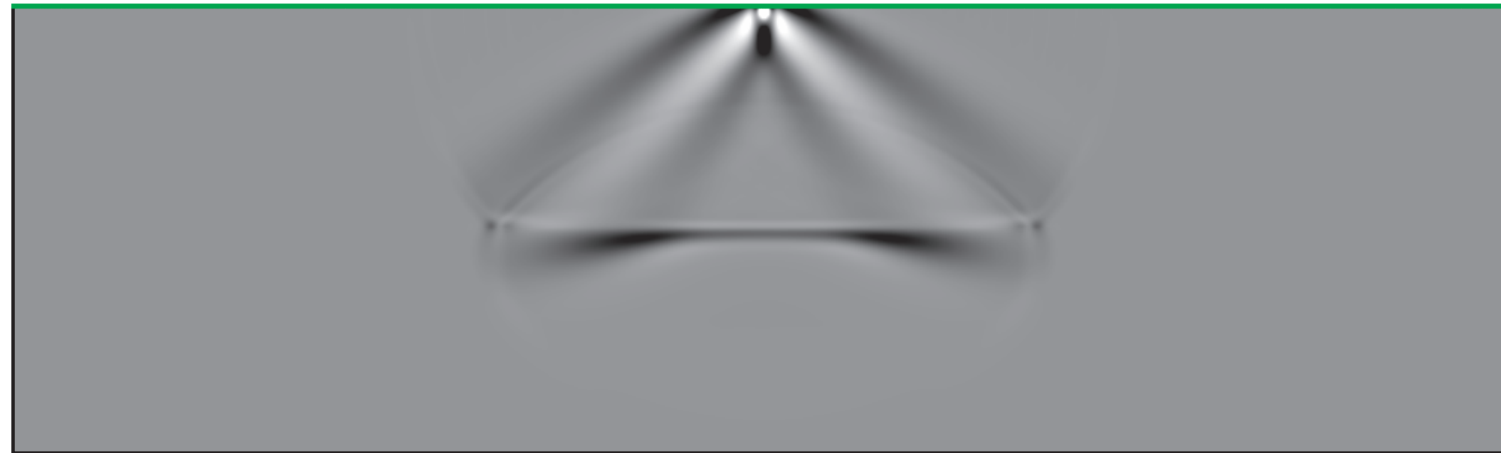
RTM image
