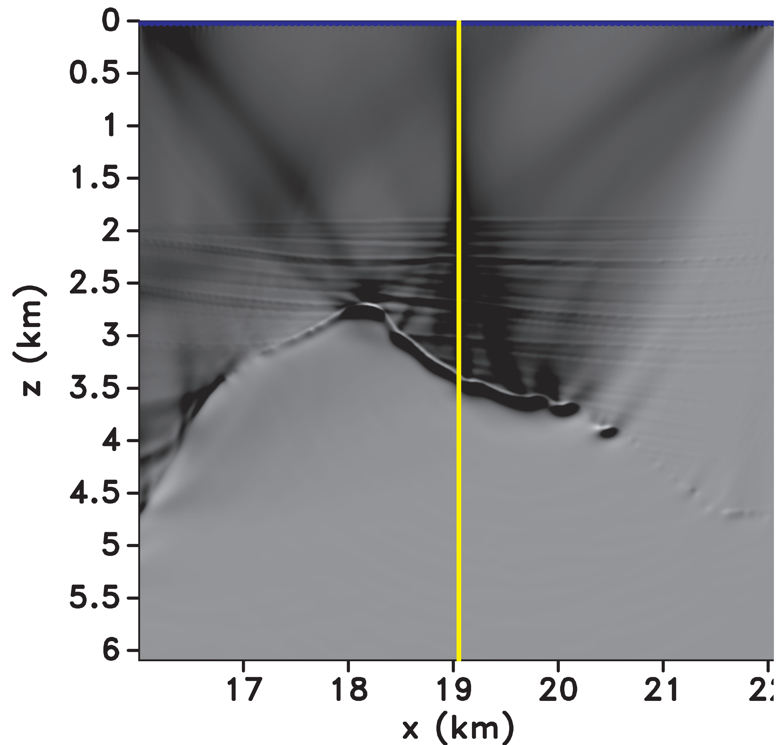
RTM image
