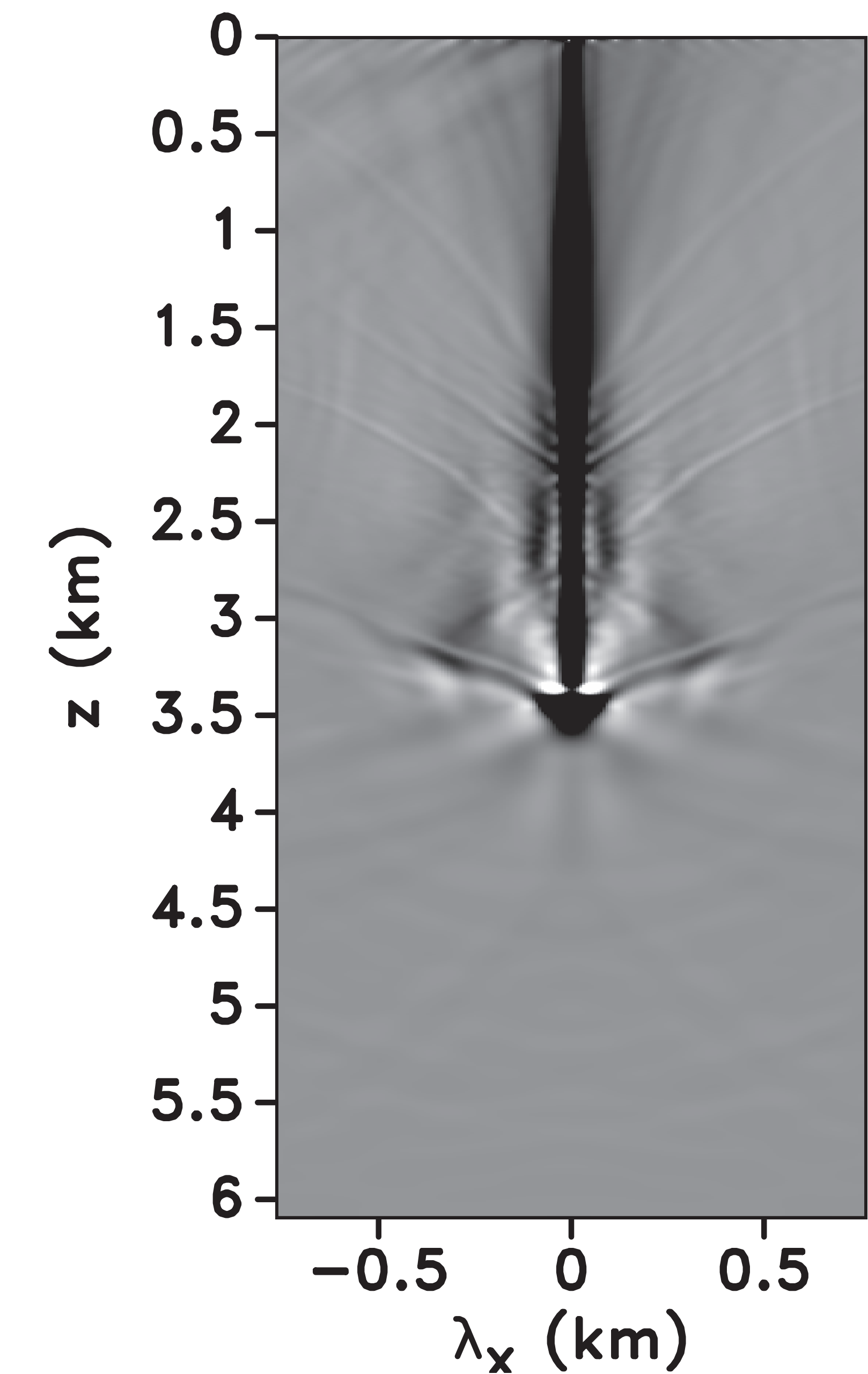
Receiver wavefield
