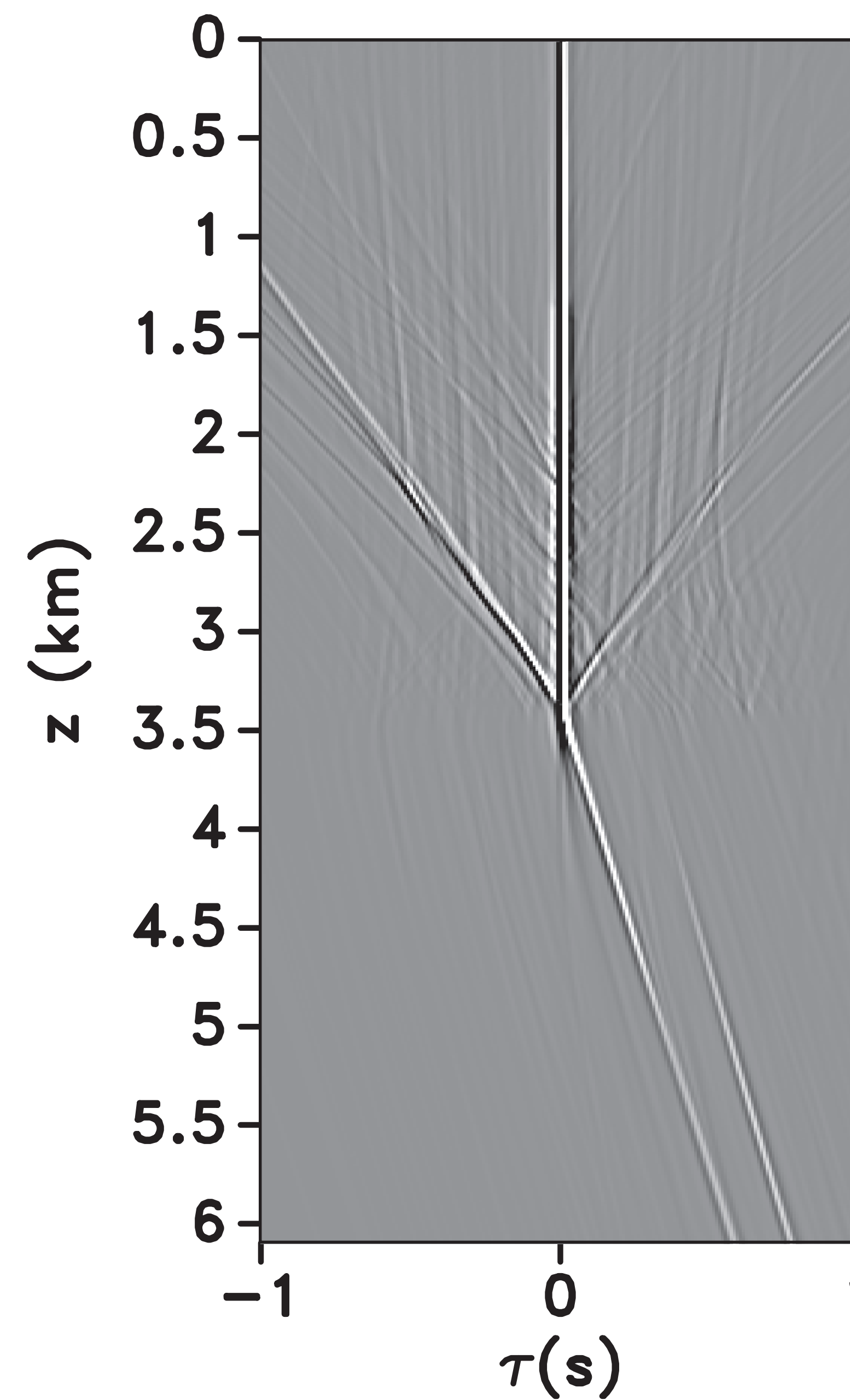
Source wavefield
