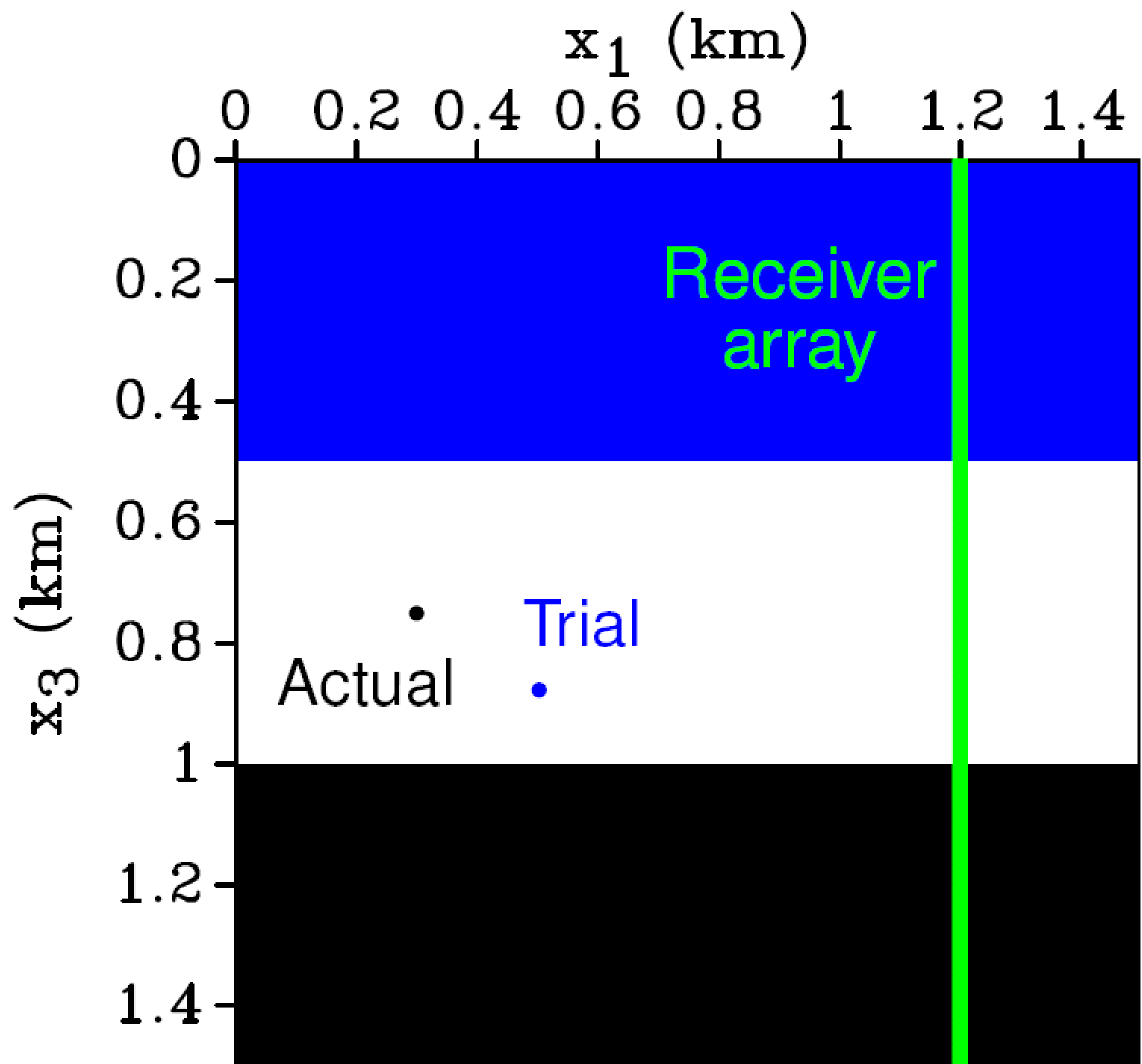
Layered model with single source
