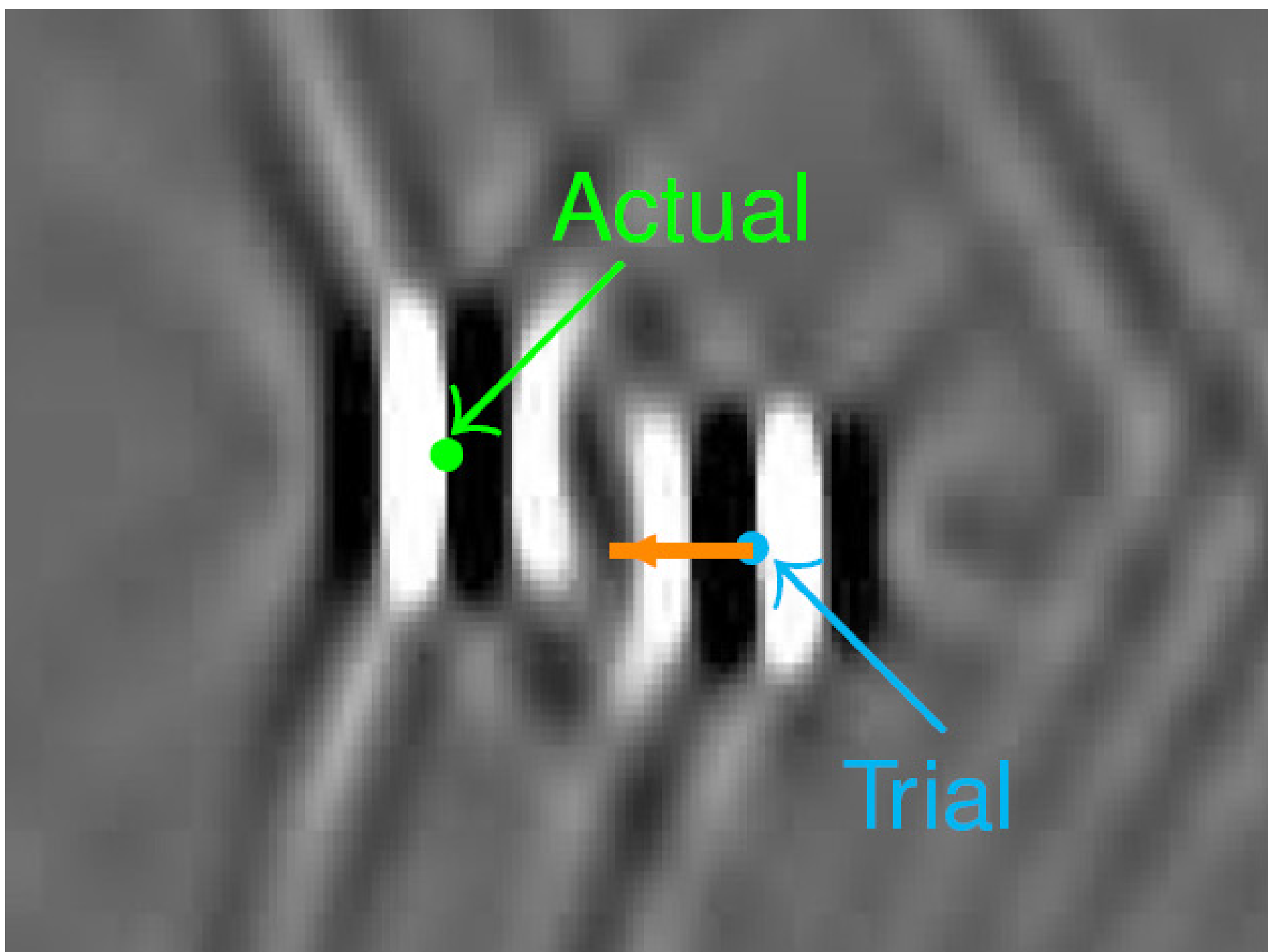
Map of \partial F / \partial x_1
