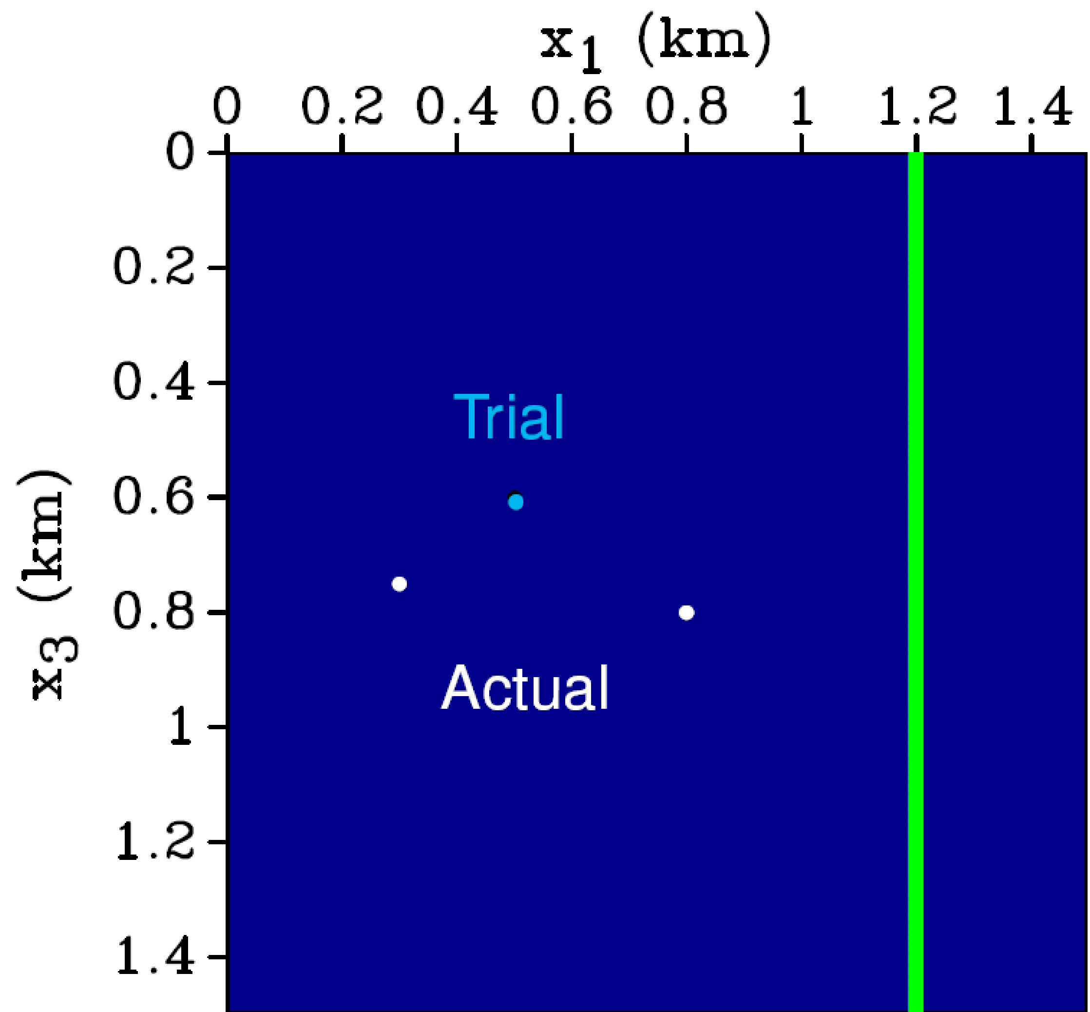
Homogeneous model with two actual sources
