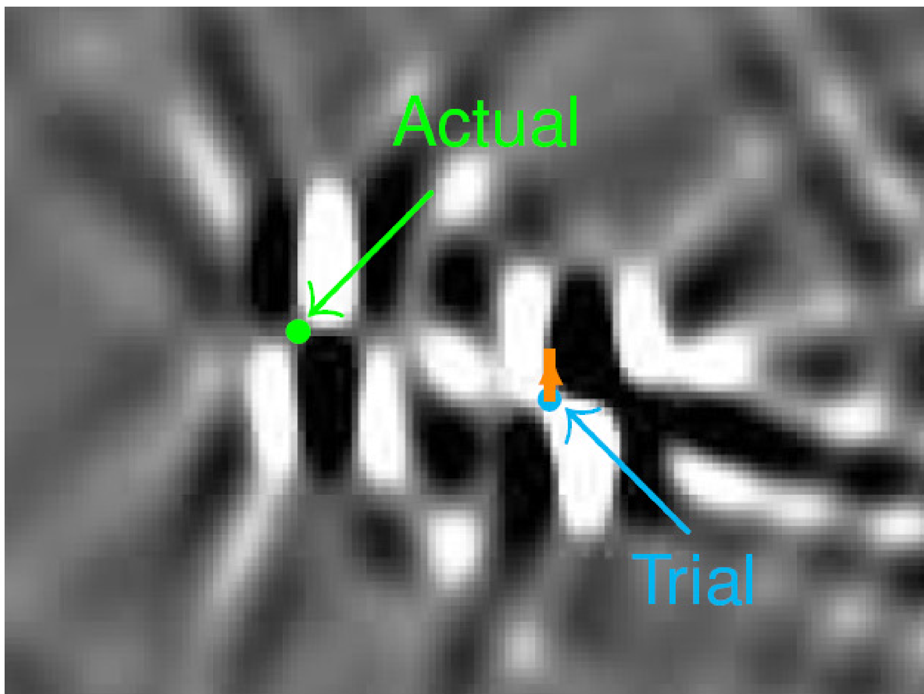
Map of \partial F / \partial x_3
