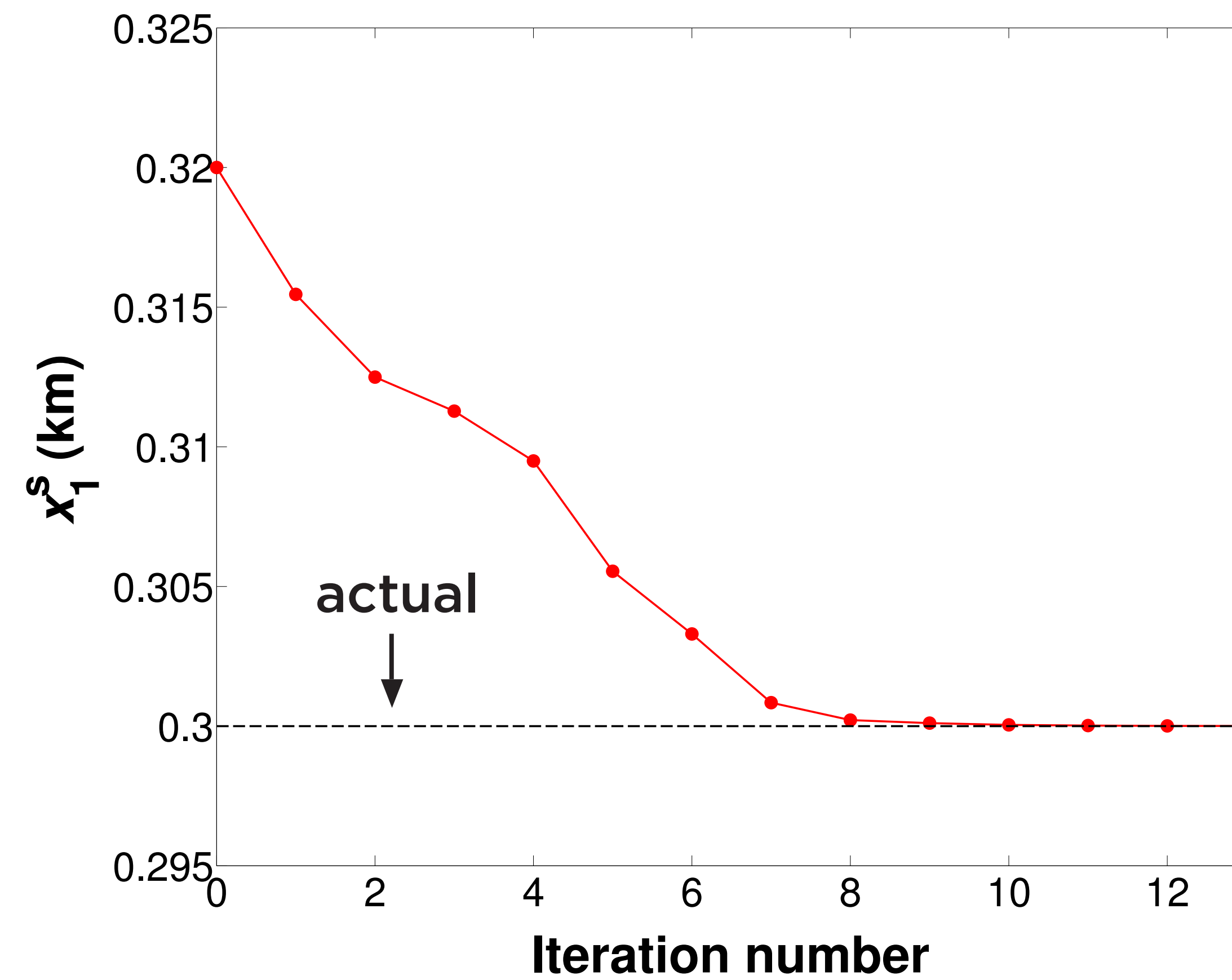
Estimation of source coordinates
