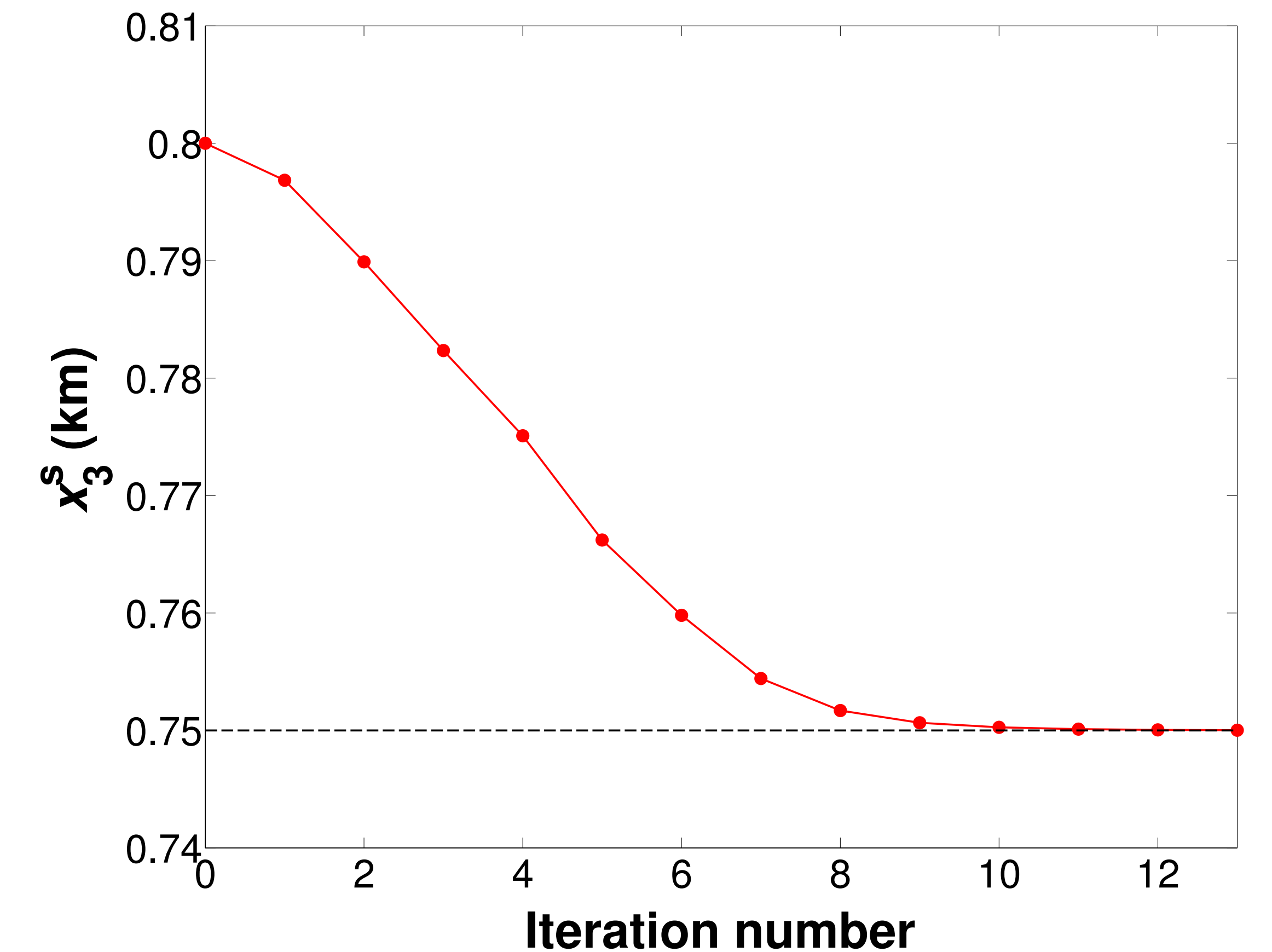
Estimation of source coordinates
