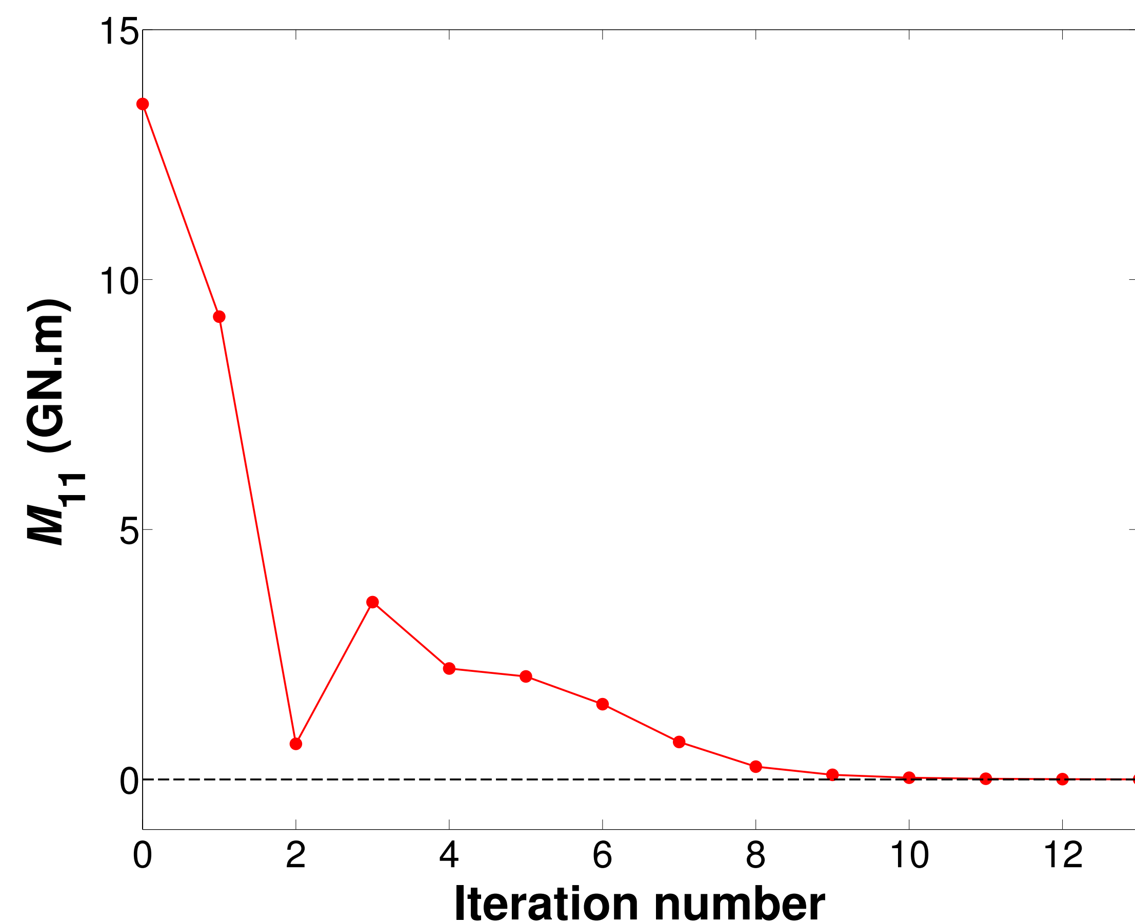
Estimation of moment tensor
