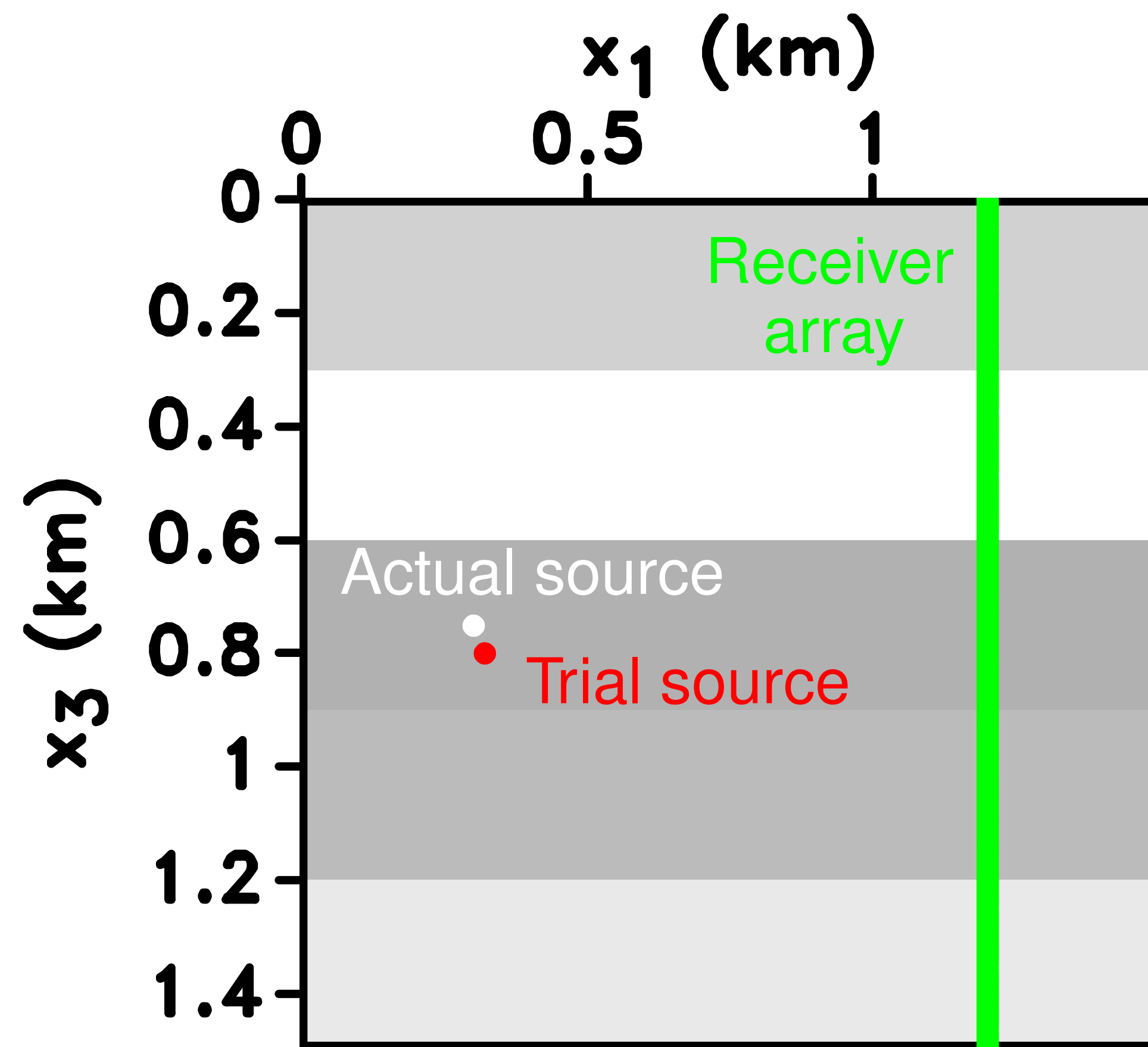
Layered VTI model
