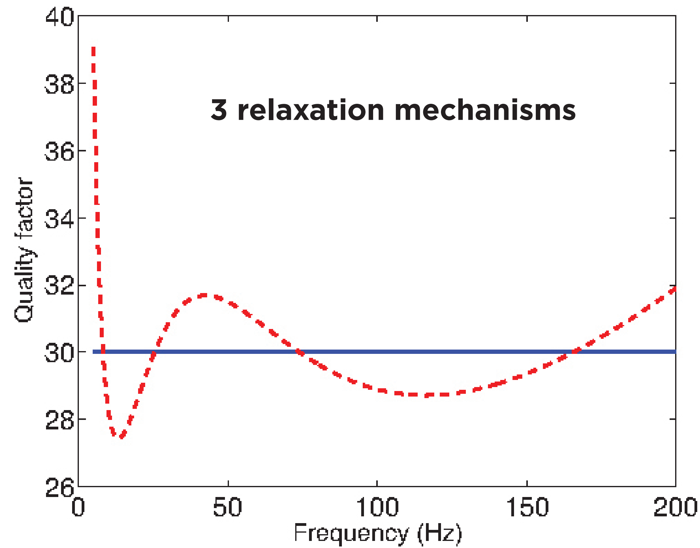
Nearly constant Q simulation
