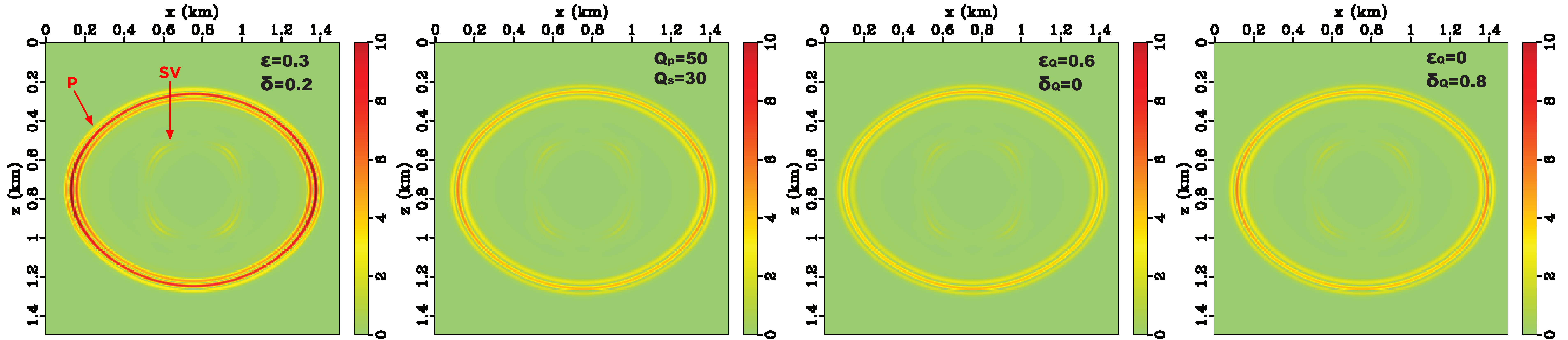
Elastic VTI
