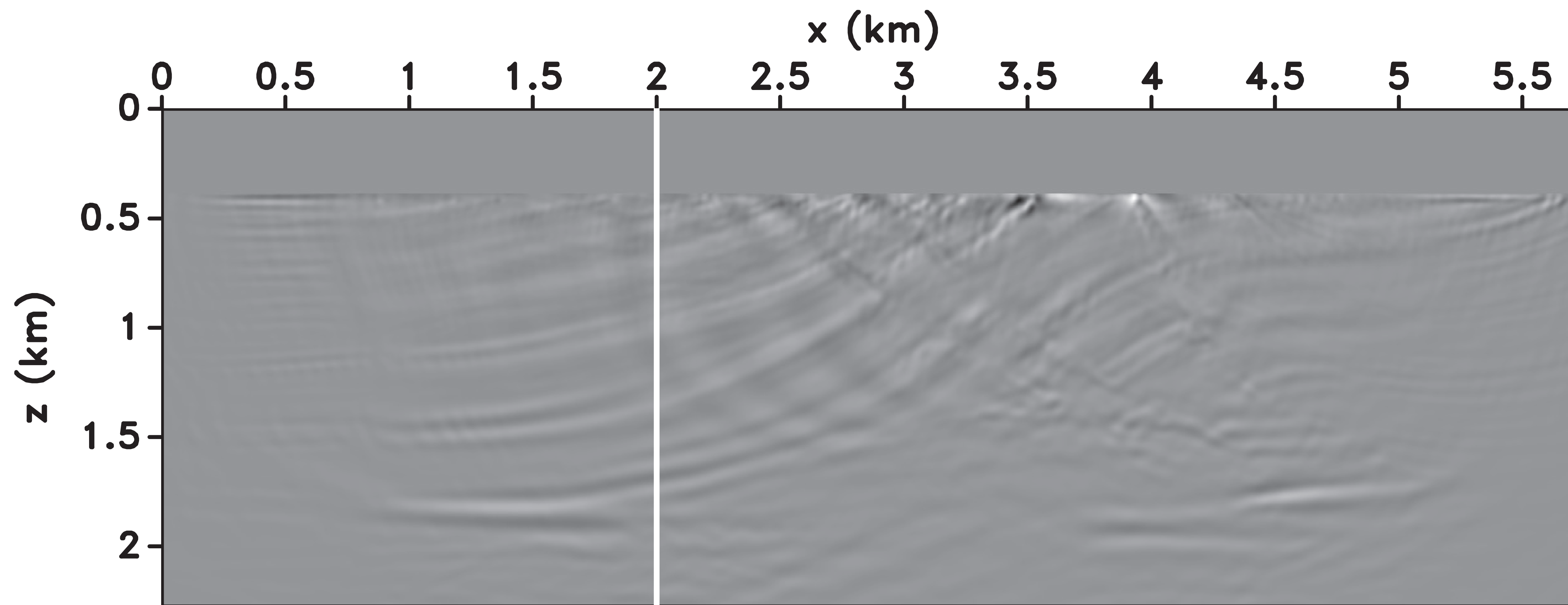
PS stack image using vector imaging condition
