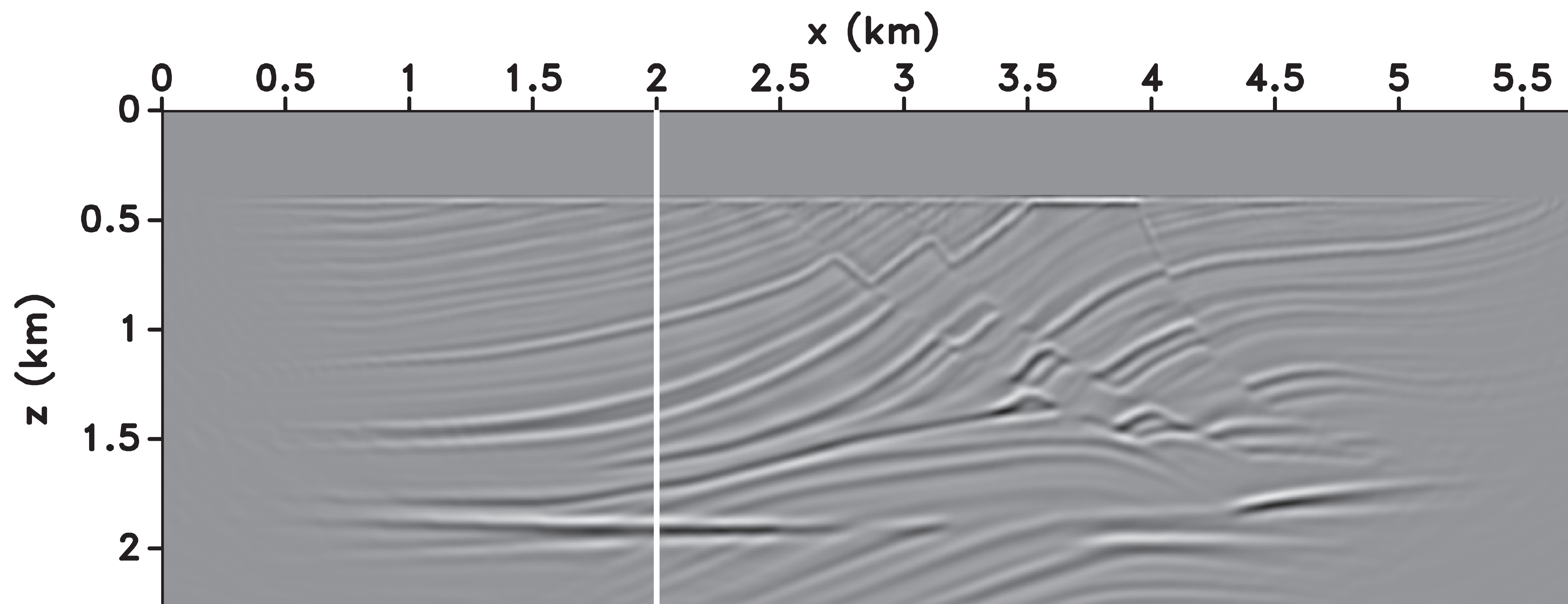
PS stack image using scalar imaging condition
